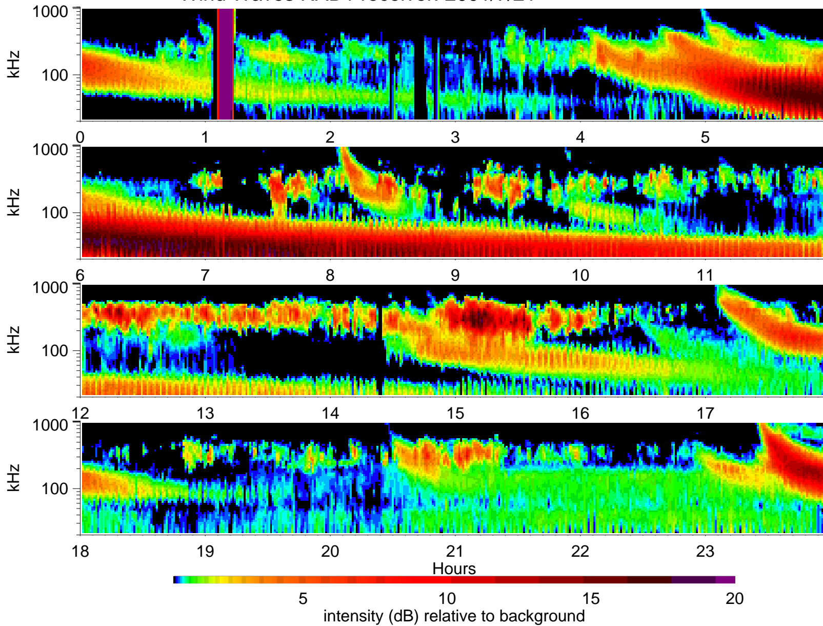
Wind Waves RAD1 receiver: 2001/7/21
