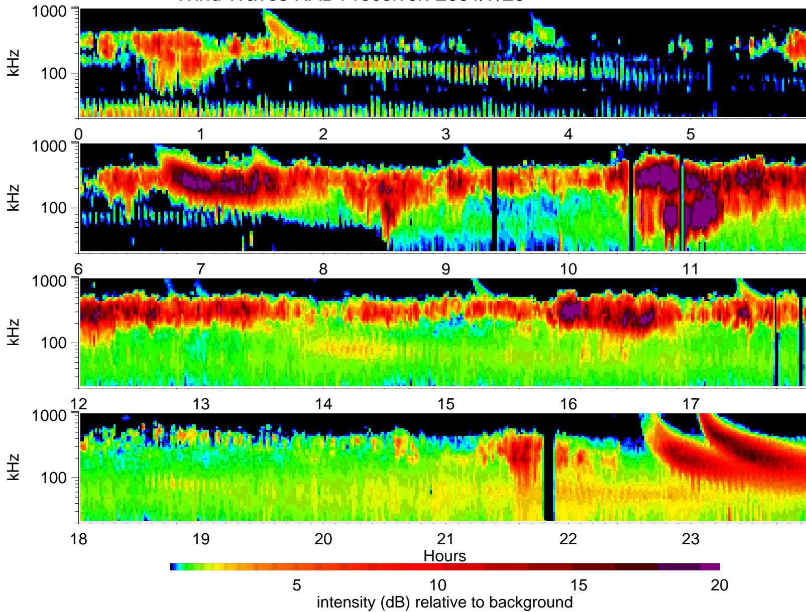
Wind Waves RAD1 receiver: 2001/7/20
