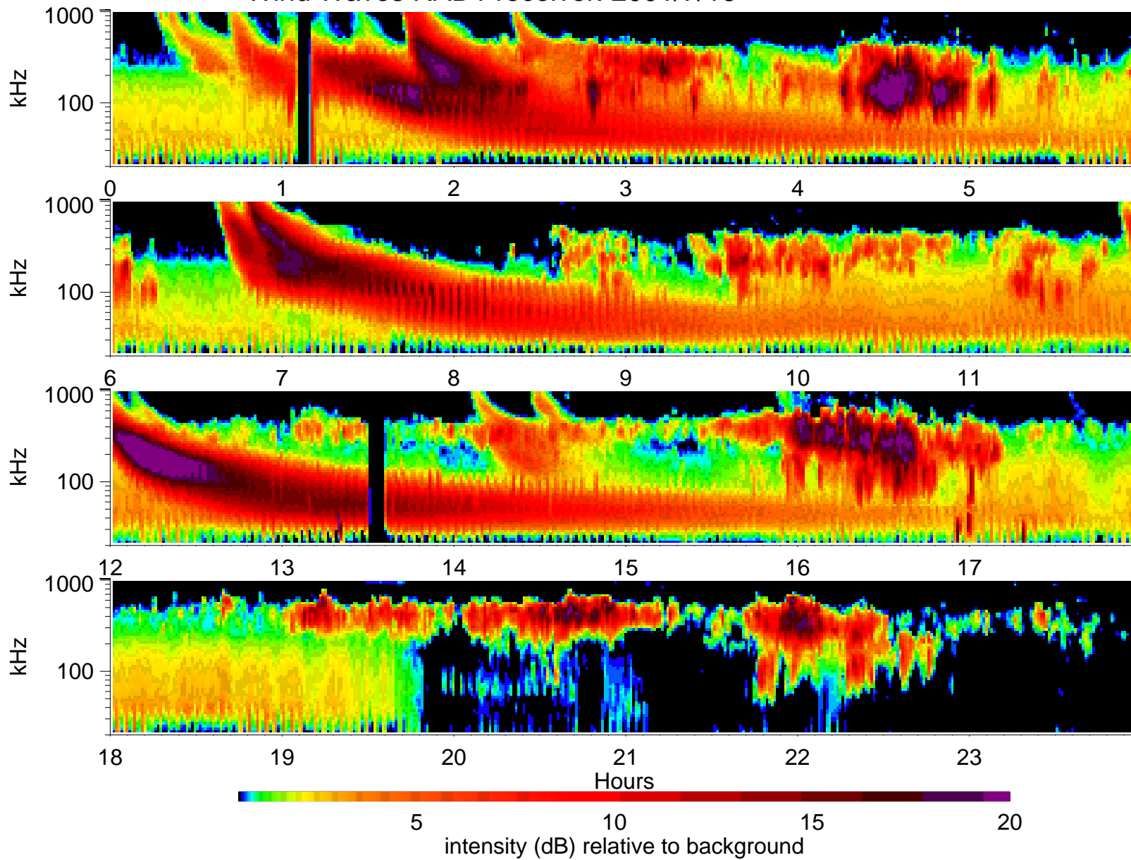
Wind Waves RAD1 receiver: 2001/7/16
