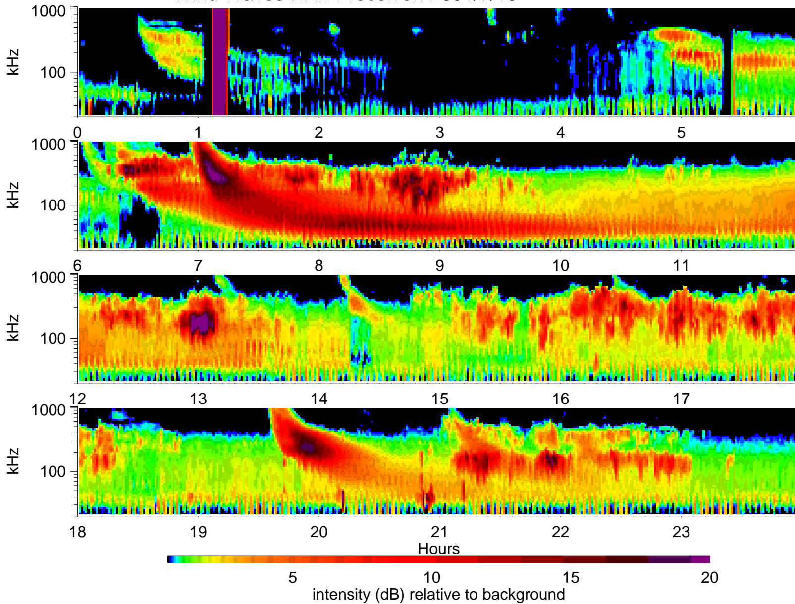
Wind Waves RAD1 receiver: 2001/7/15
