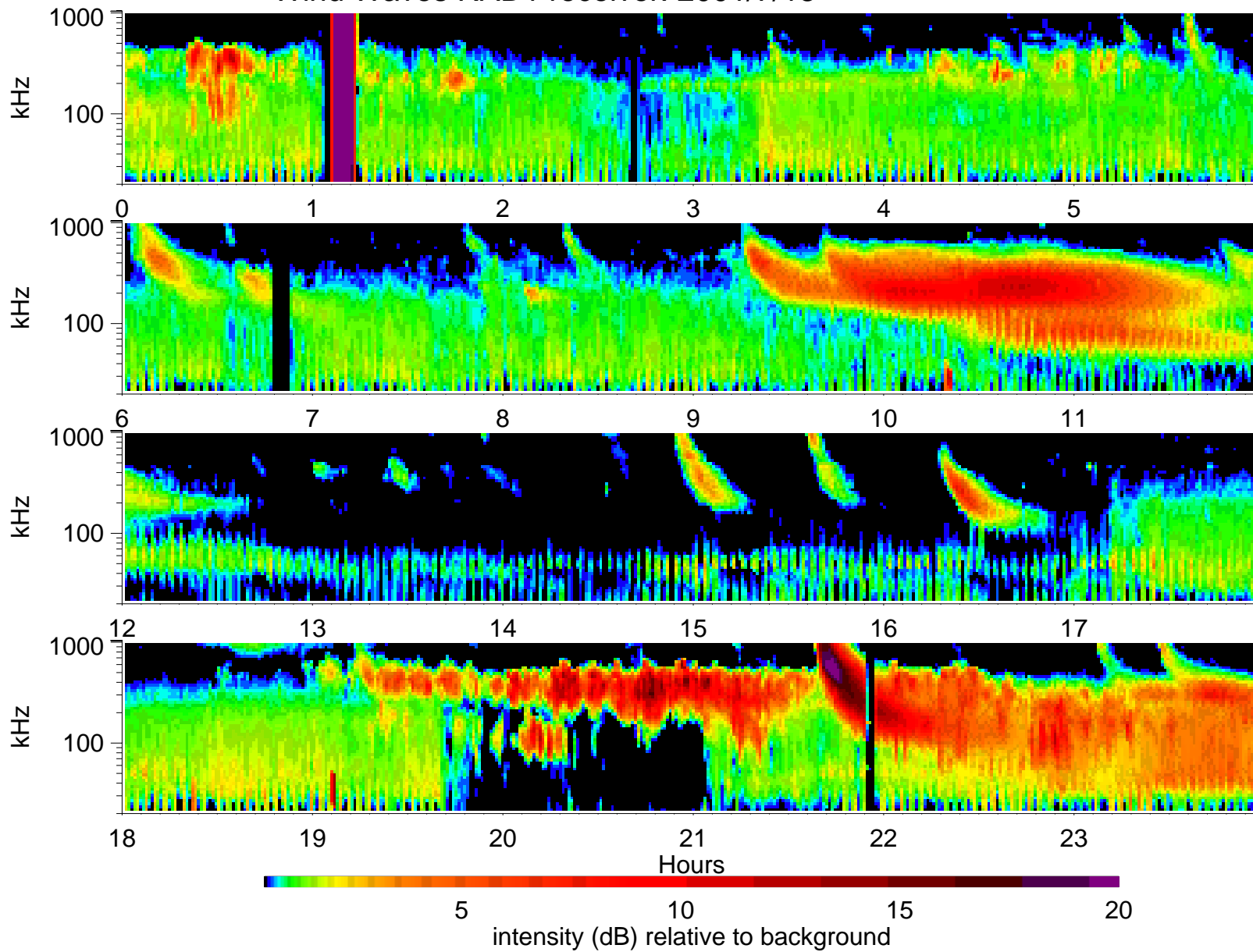
Wind Waves RAD1 receiver: 2001/7/13
