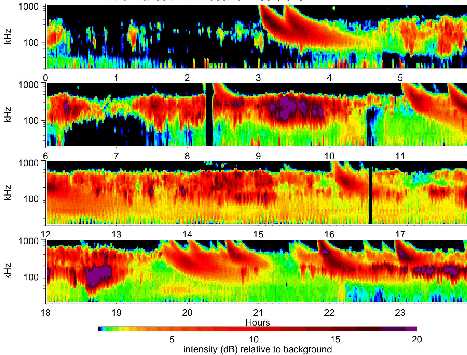
Wind Waves RAD1 receiver: 2001/7/10
