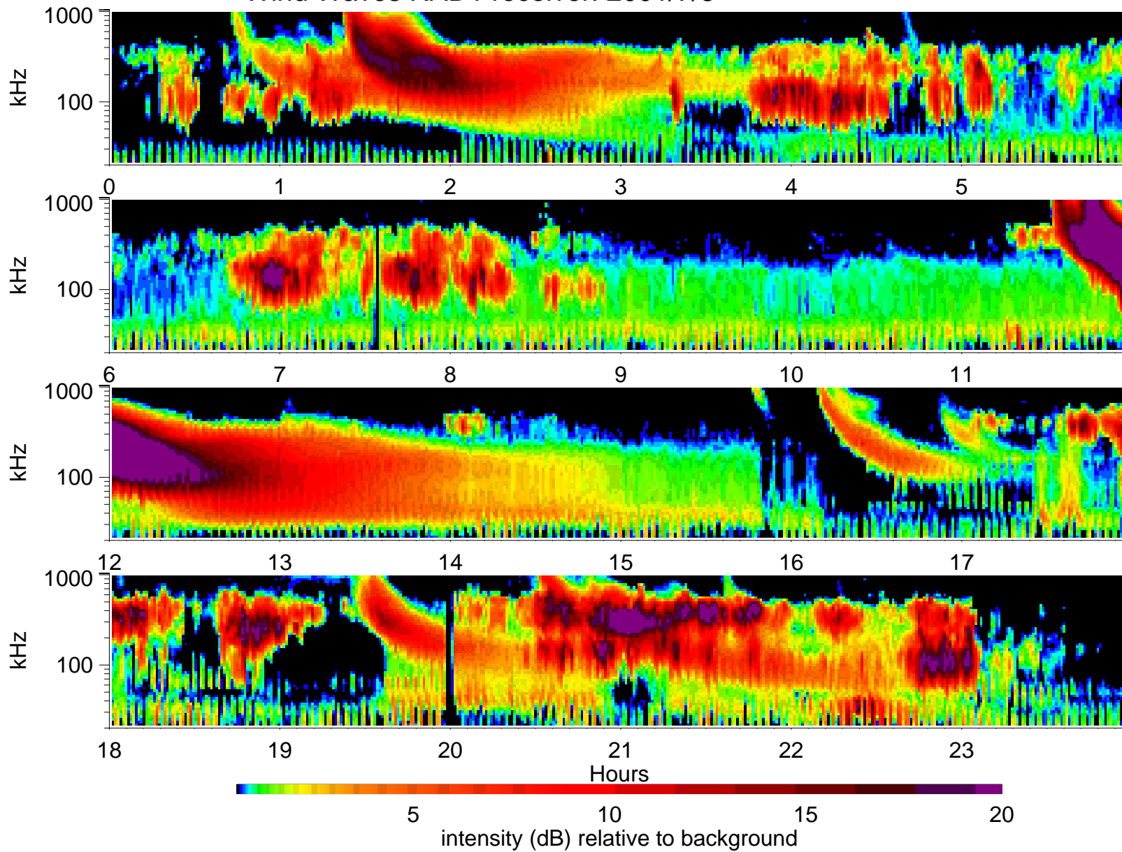
Wind Waves RAD1 receiver: 2001/7/8
