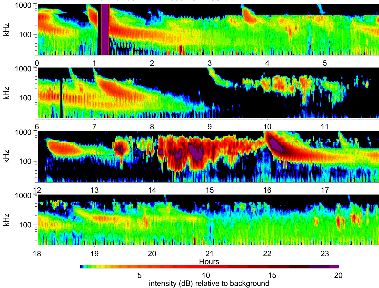
Wind Waves RAD1 receiver: 2001/7/7
