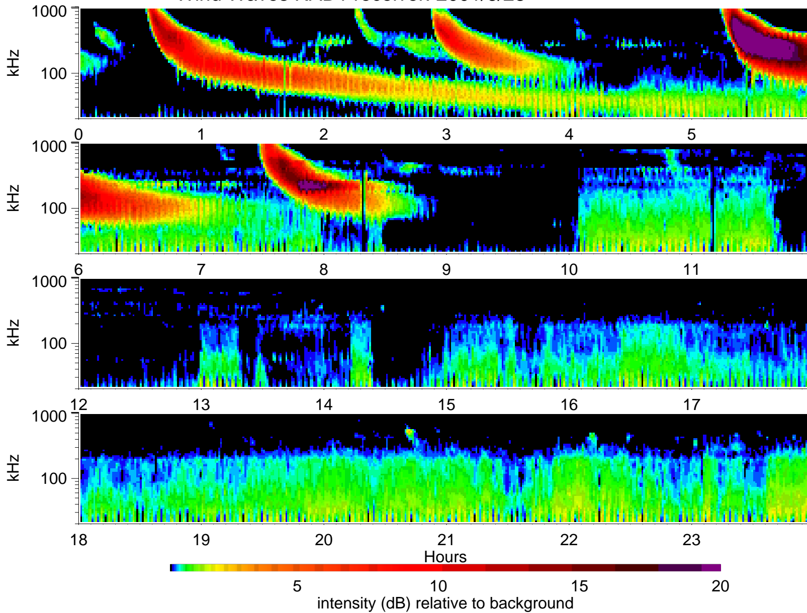
Wind Waves RAD1 receiver: 2001/6/28
