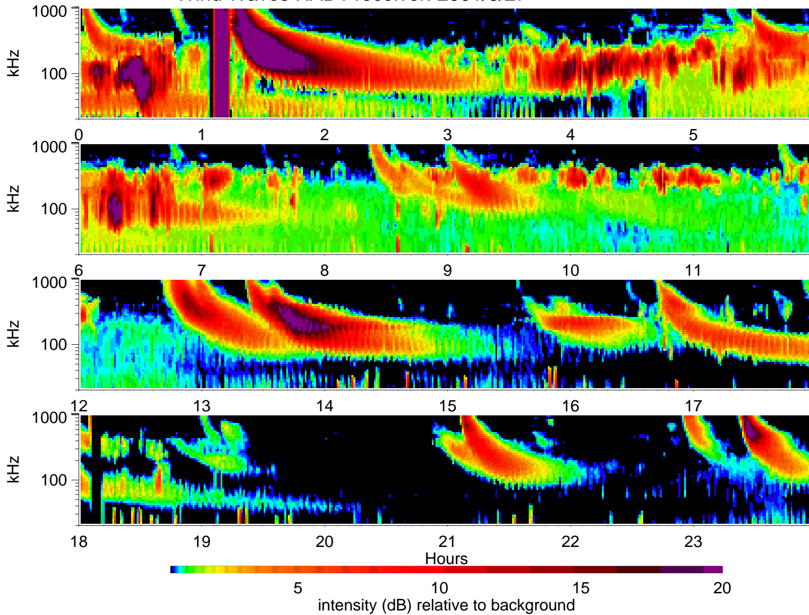
Wind Waves RAD1 receiver: 2001/6/27
