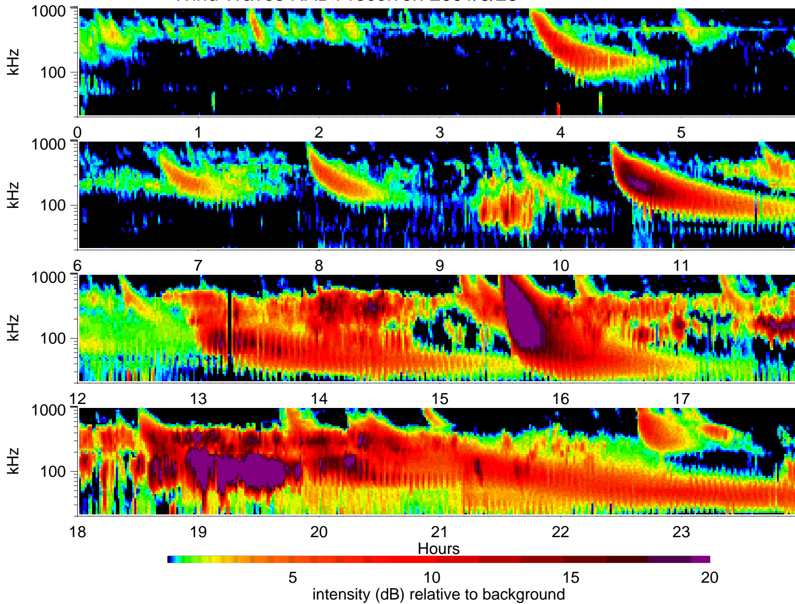
Wind Waves RAD1 receiver: 2001/6/26
