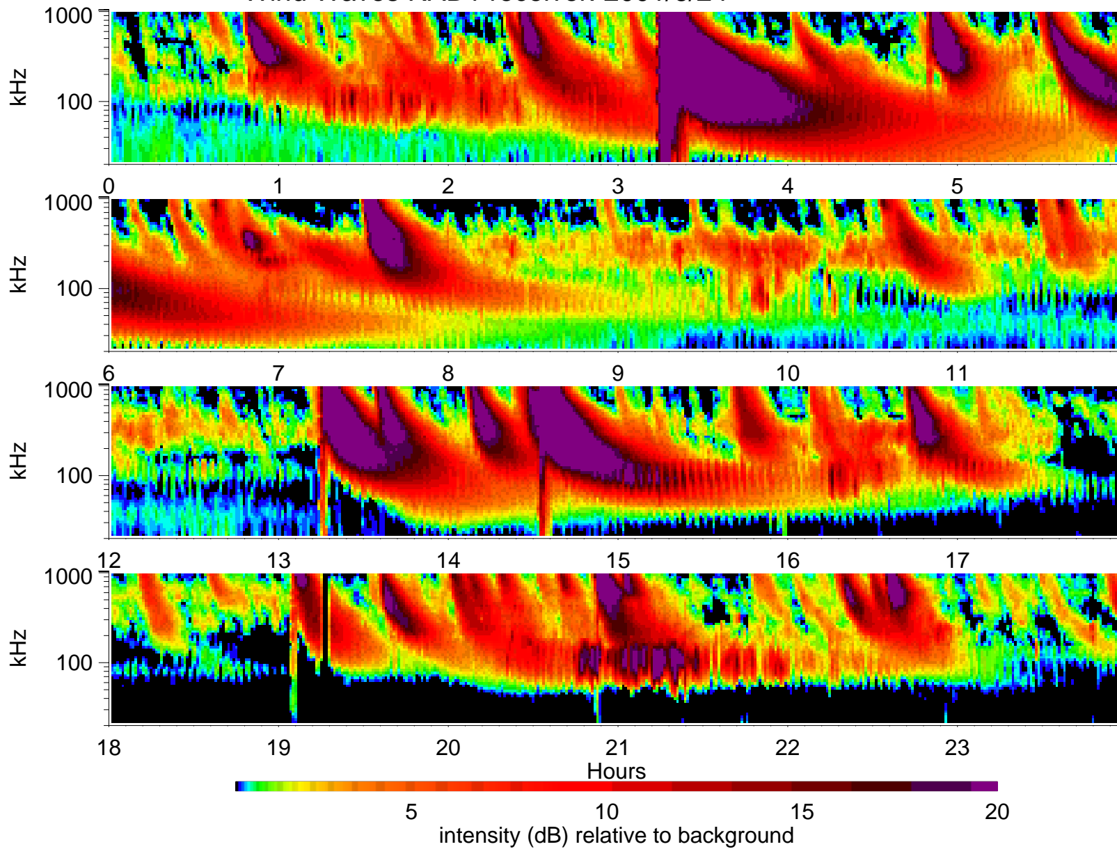
Wind Waves RAD1 receiver: 2001/6/24
