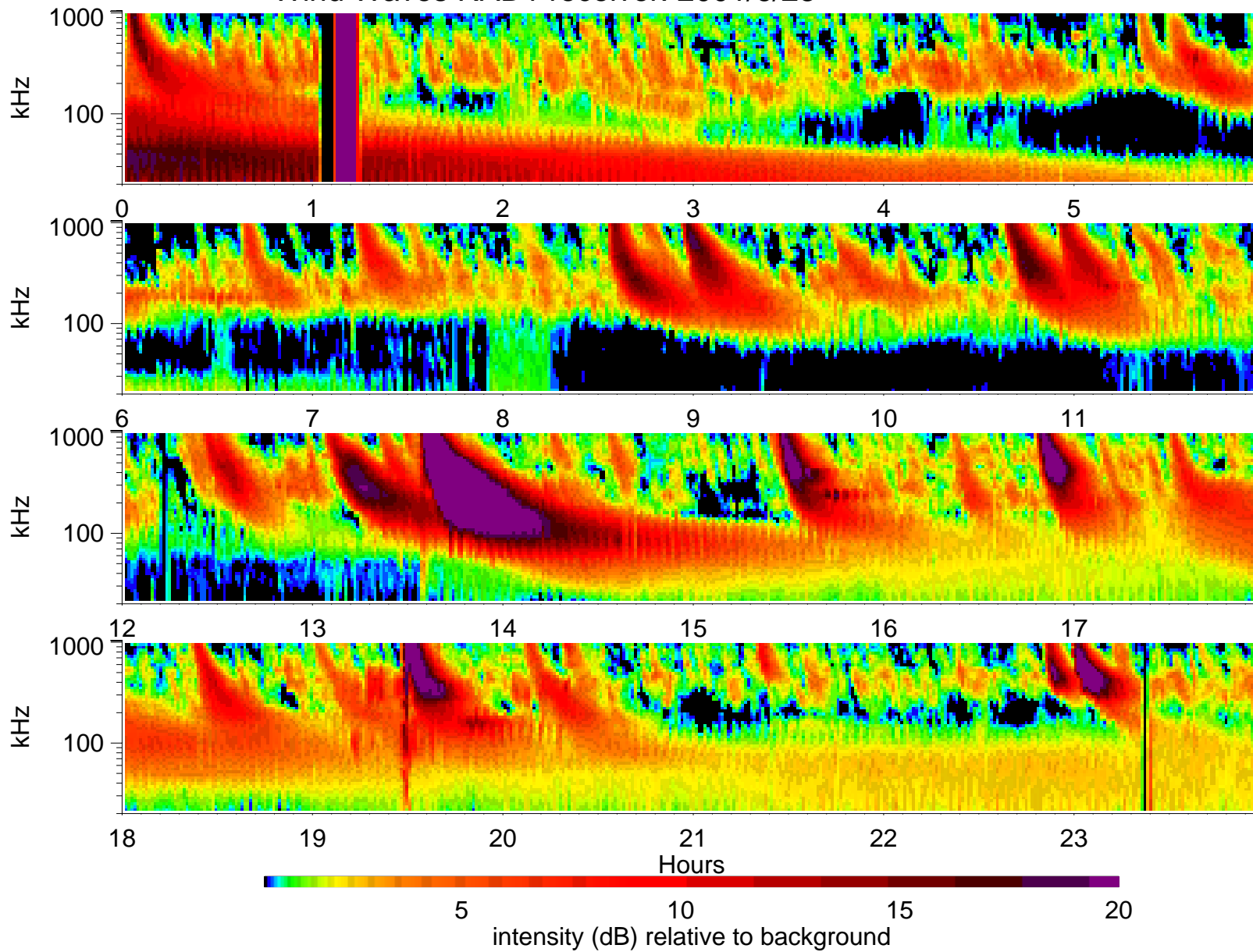
Wind Waves RAD1 receiver: 2001/6/23
