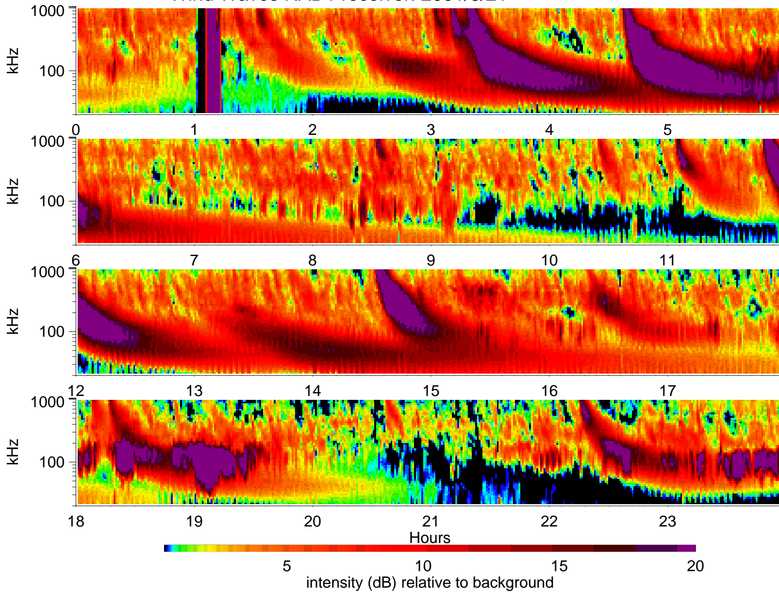
Wind Waves RAD1 receiver: 2001/6/21
