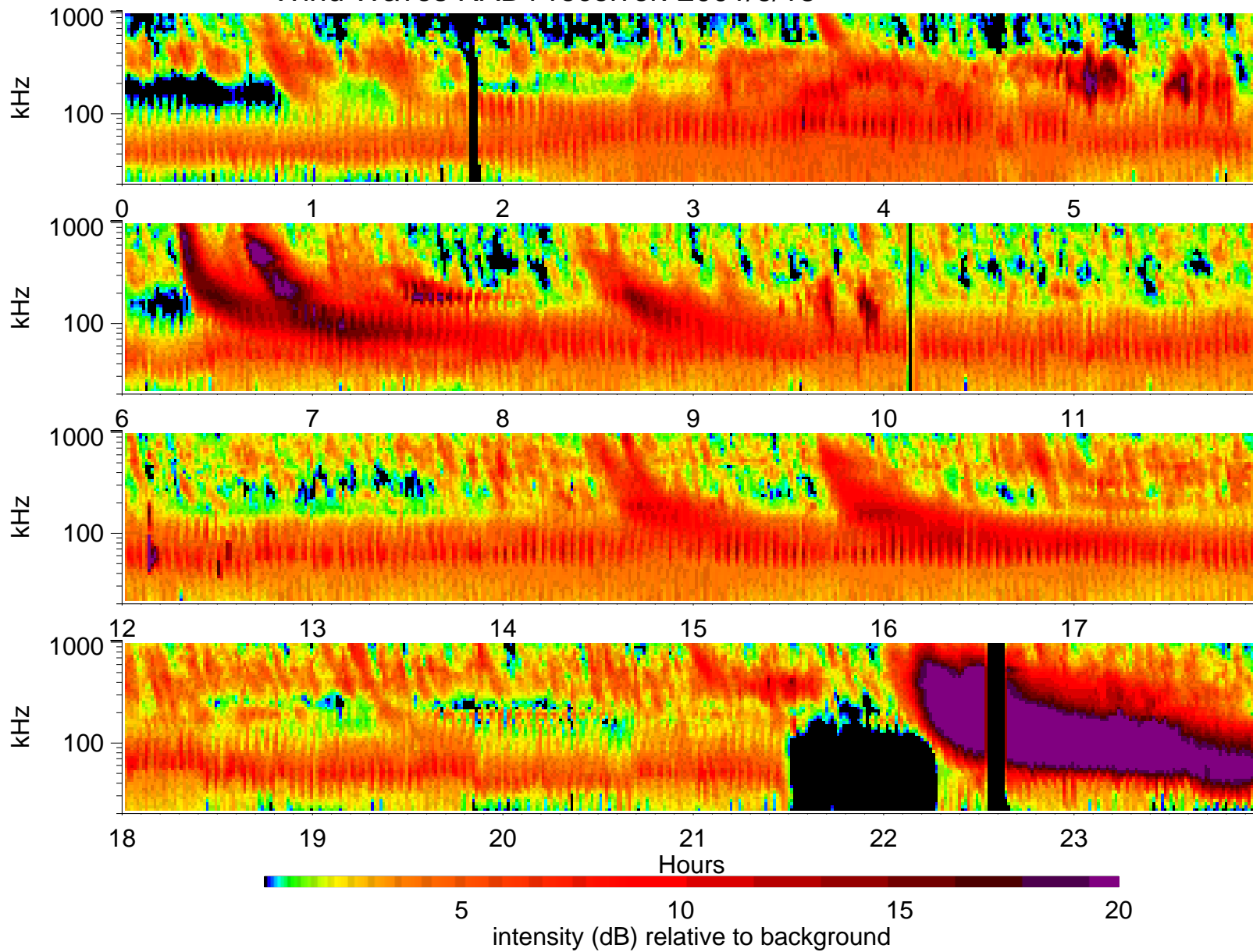
Wind Waves RAD1 receiver: 2001/6/18
