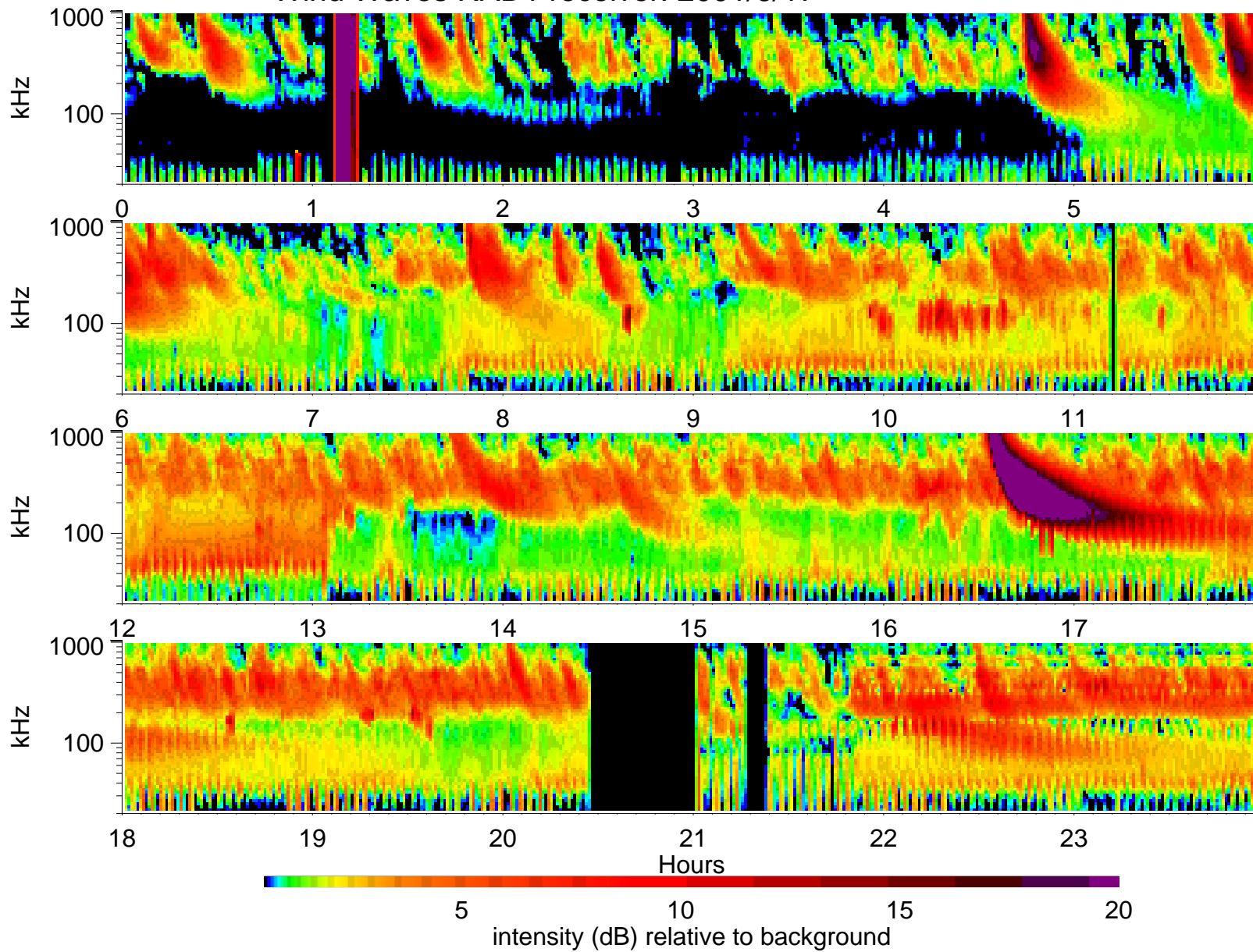
Wind Waves RAD1 receiver: 2001/6/17
