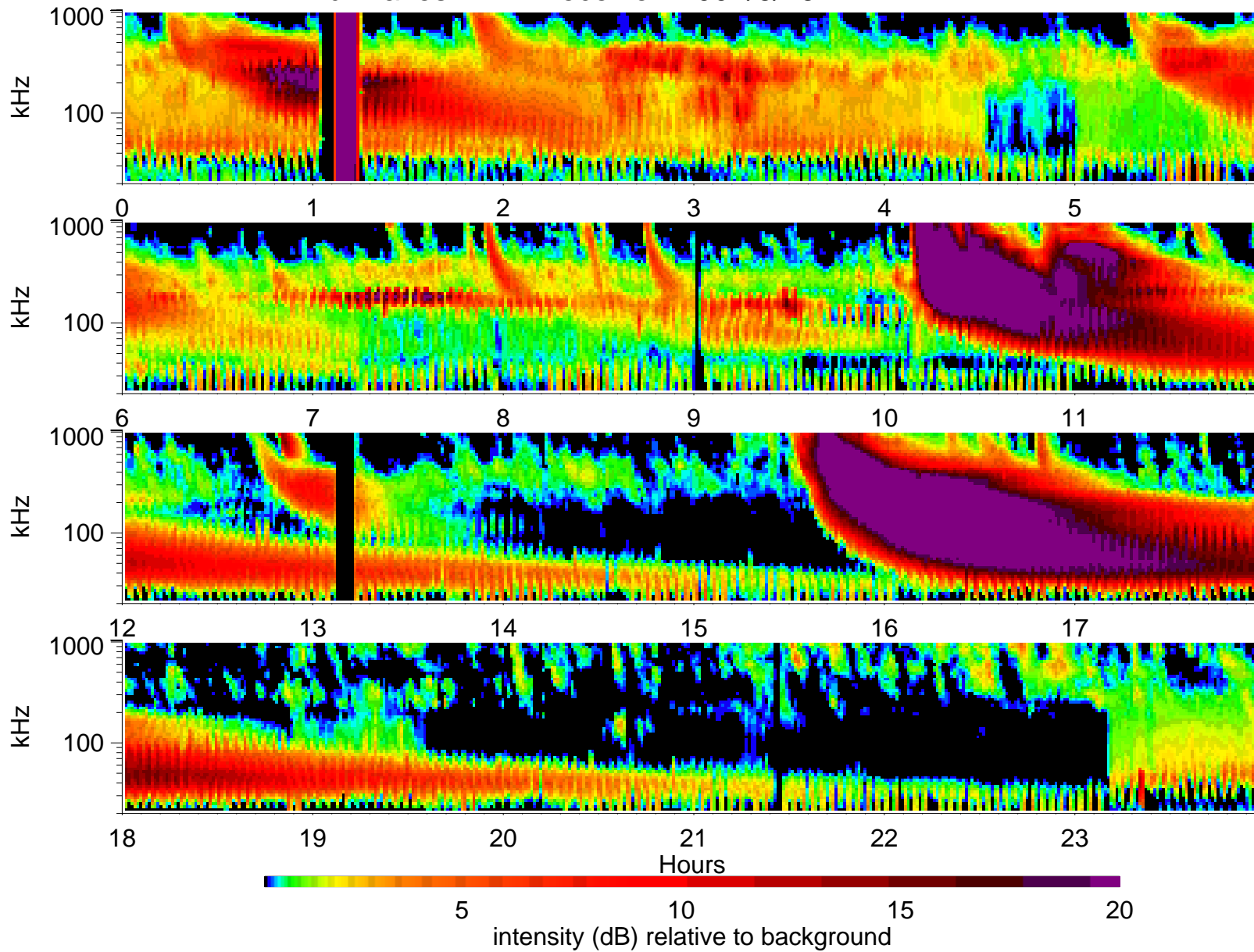
Wind Waves RAD1 receiver: 2001/6/15
