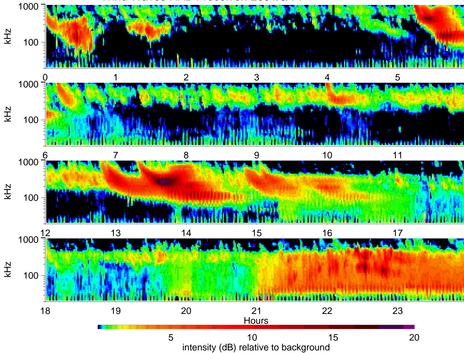
Wind Waves RAD1 receiver: 2001/6/14
