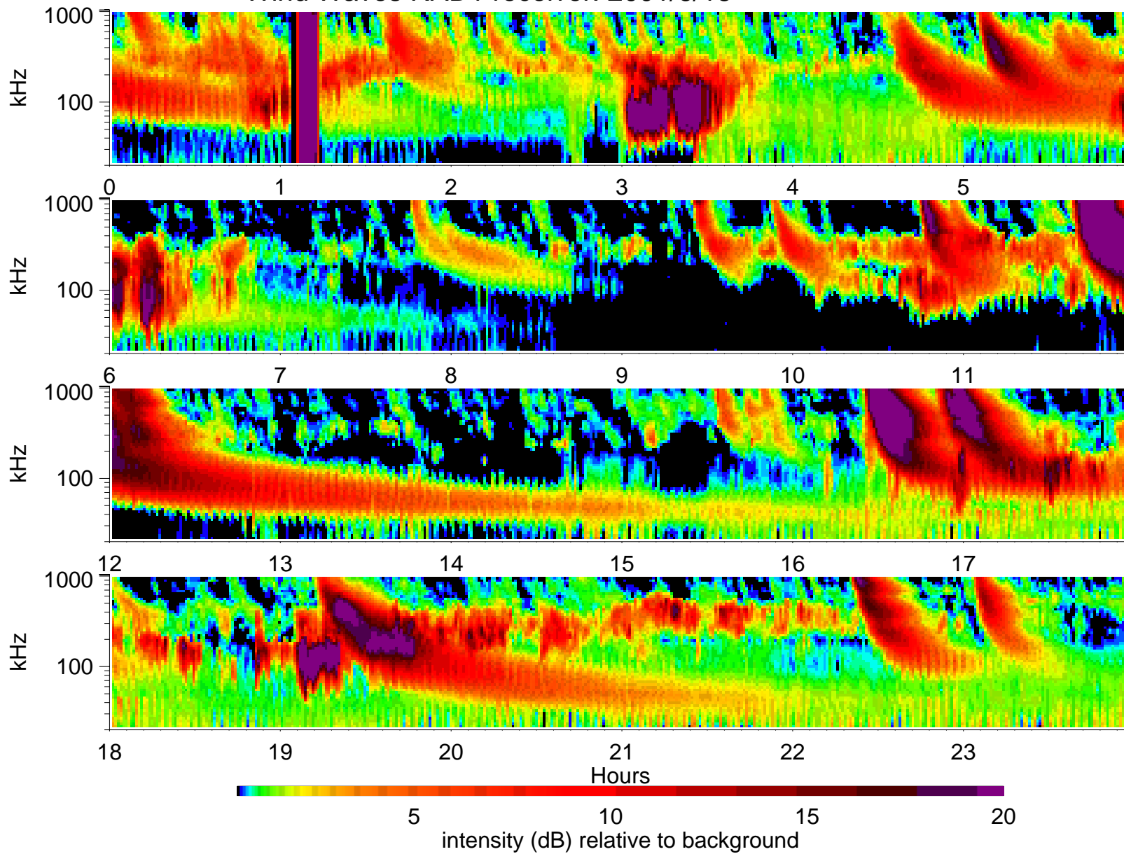
Wind Waves RAD1 receiver: 2001/6/13
