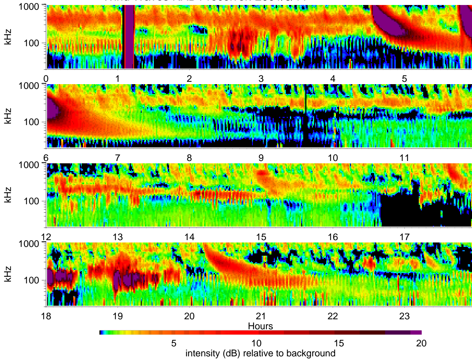
Wind Waves RAD1 receiver: 2001/6/11
