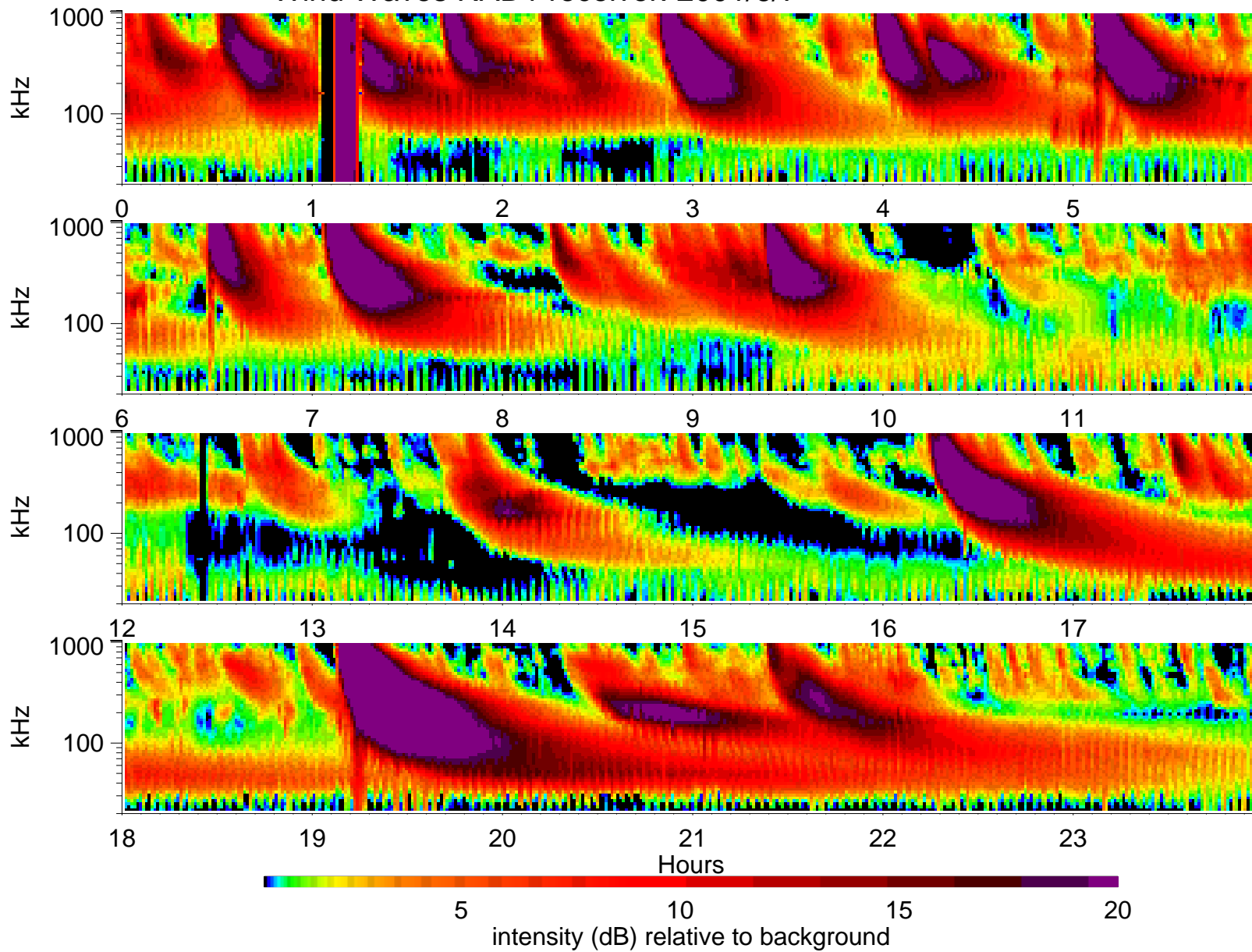
Wind Waves RAD1 receiver: 2001/6/7
