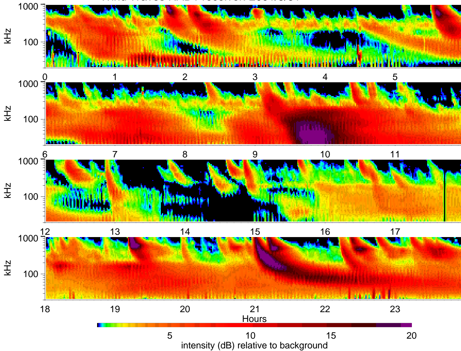
Wind Waves RAD1 receiver: 2001/5/31
