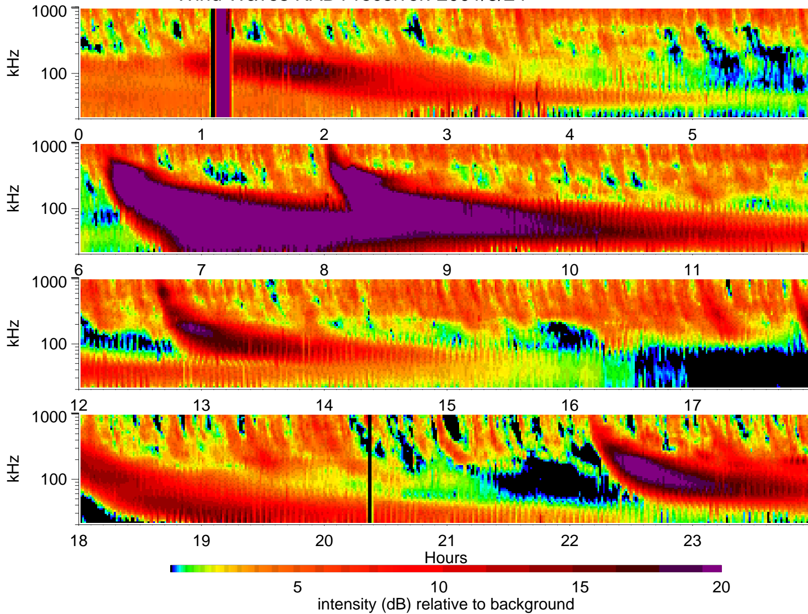
Wind Waves RAD1 receiver: 2001/5/24
