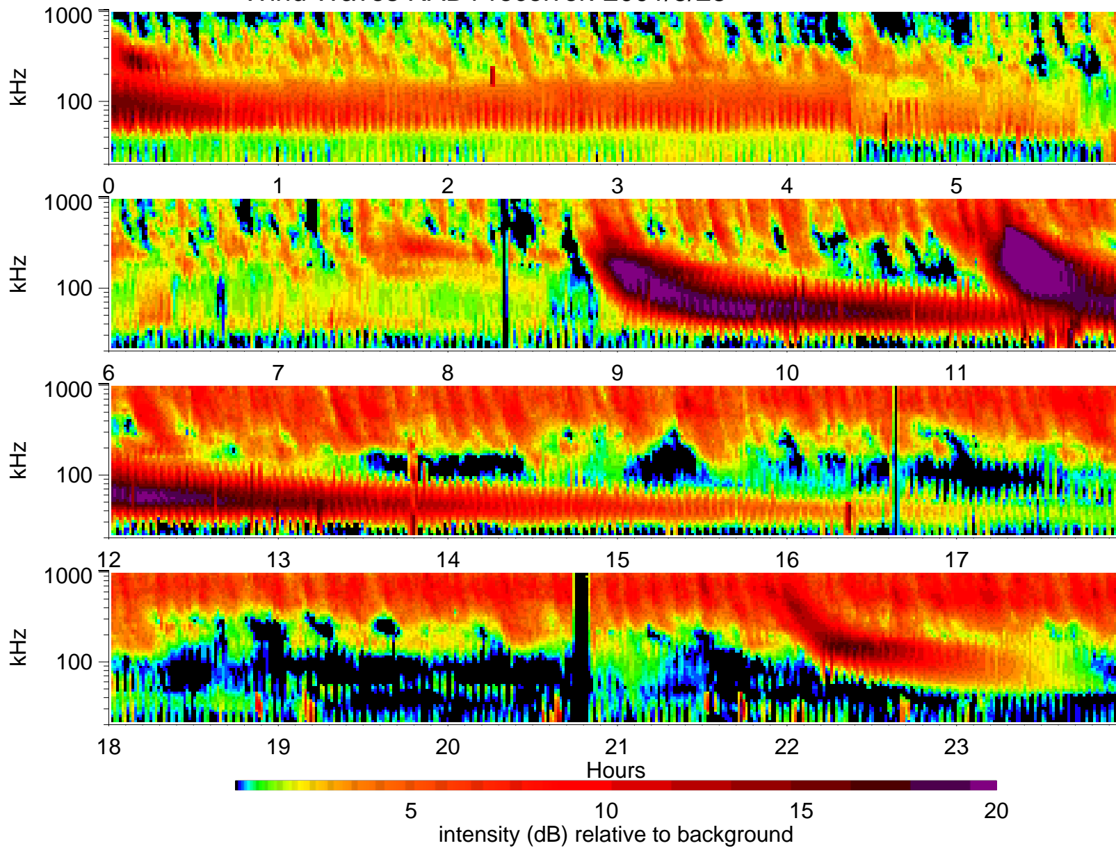
Wind Waves RAD1 receiver: 2001/5/23
