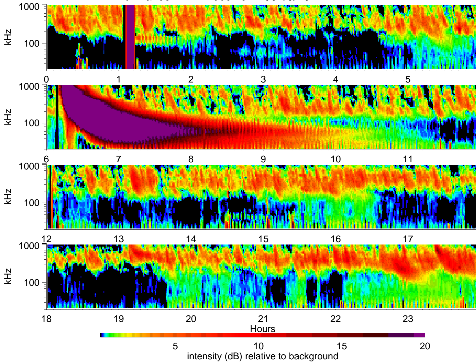
Wind Waves RAD1 receiver: 2001/5/20
