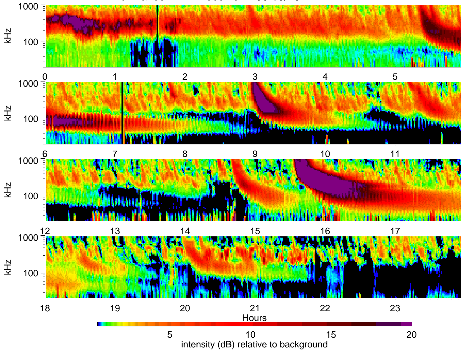
Wind Waves RAD1 receiver: 2001/5/19
