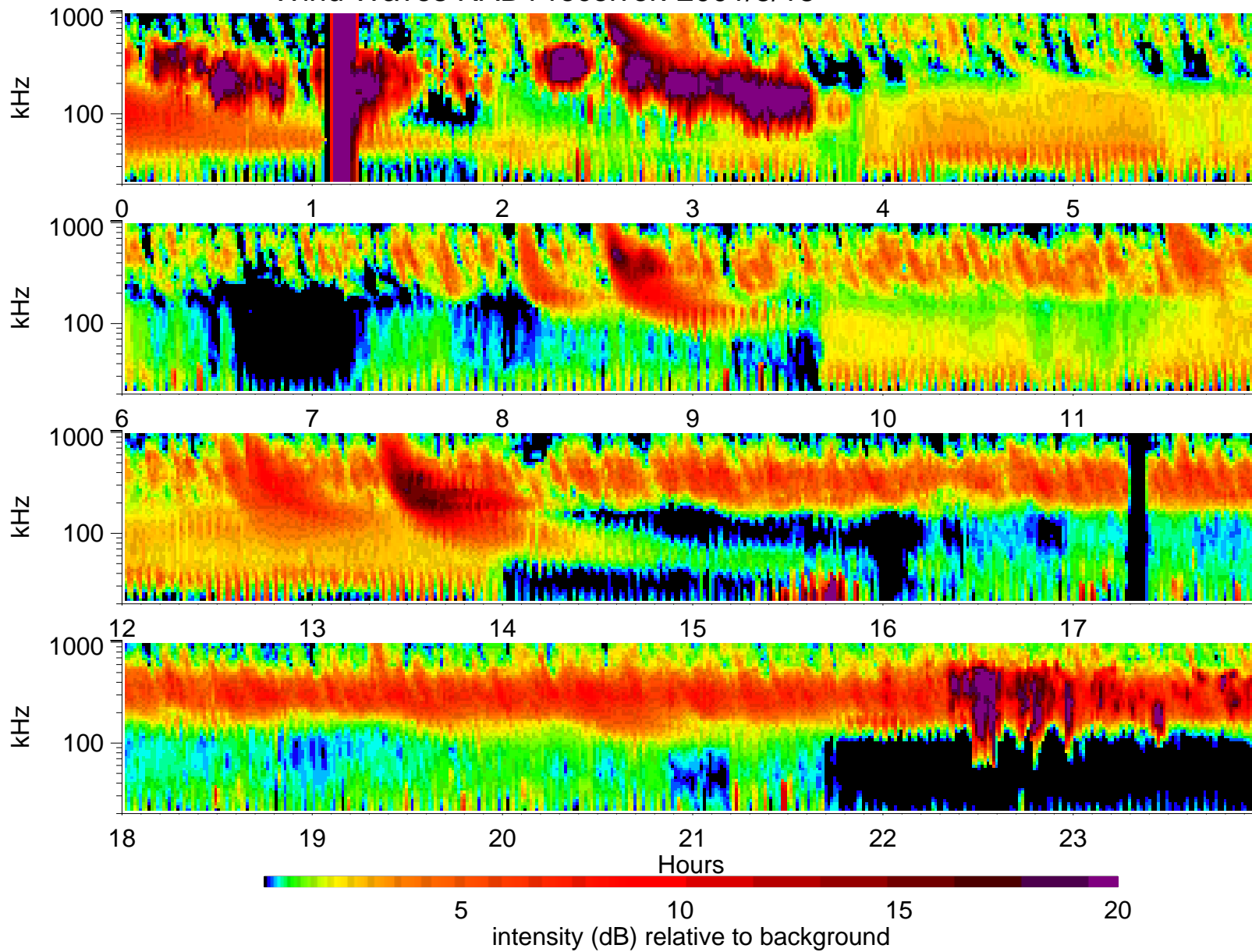
Wind Waves RAD1 receiver: 2001/5/18
