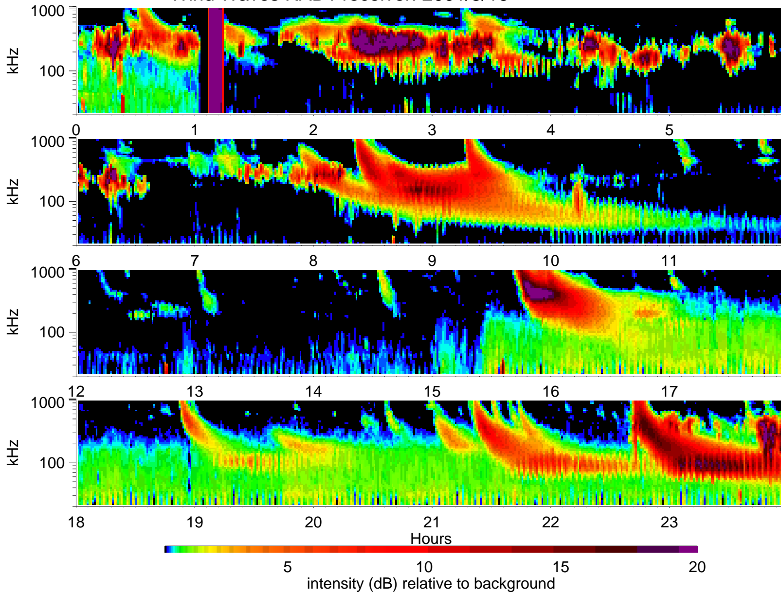
Wind Waves RAD1 receiver: 2001/5/16
