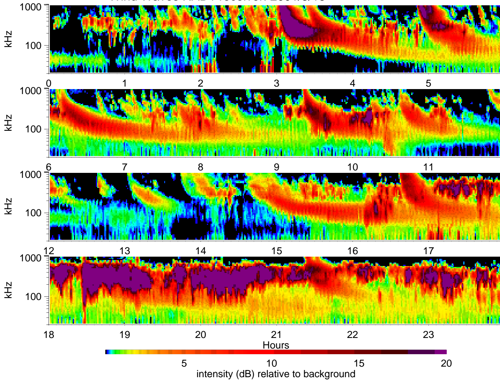
Wind Waves RAD1 receiver: 2001/5/15
