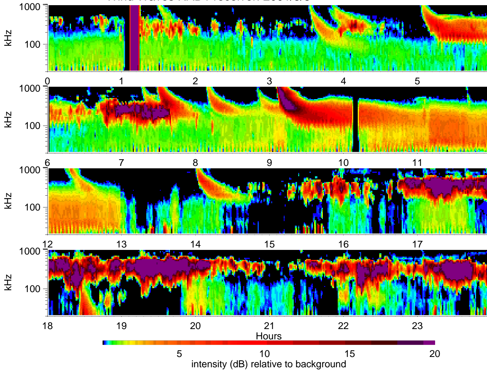
Wind Waves RAD1 receiver: 2001/5/8
