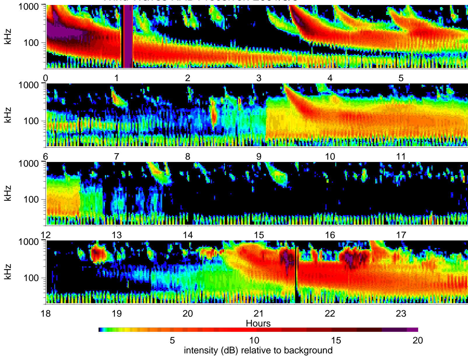
Wind Waves RAD1 receiver: 2001/5/6
