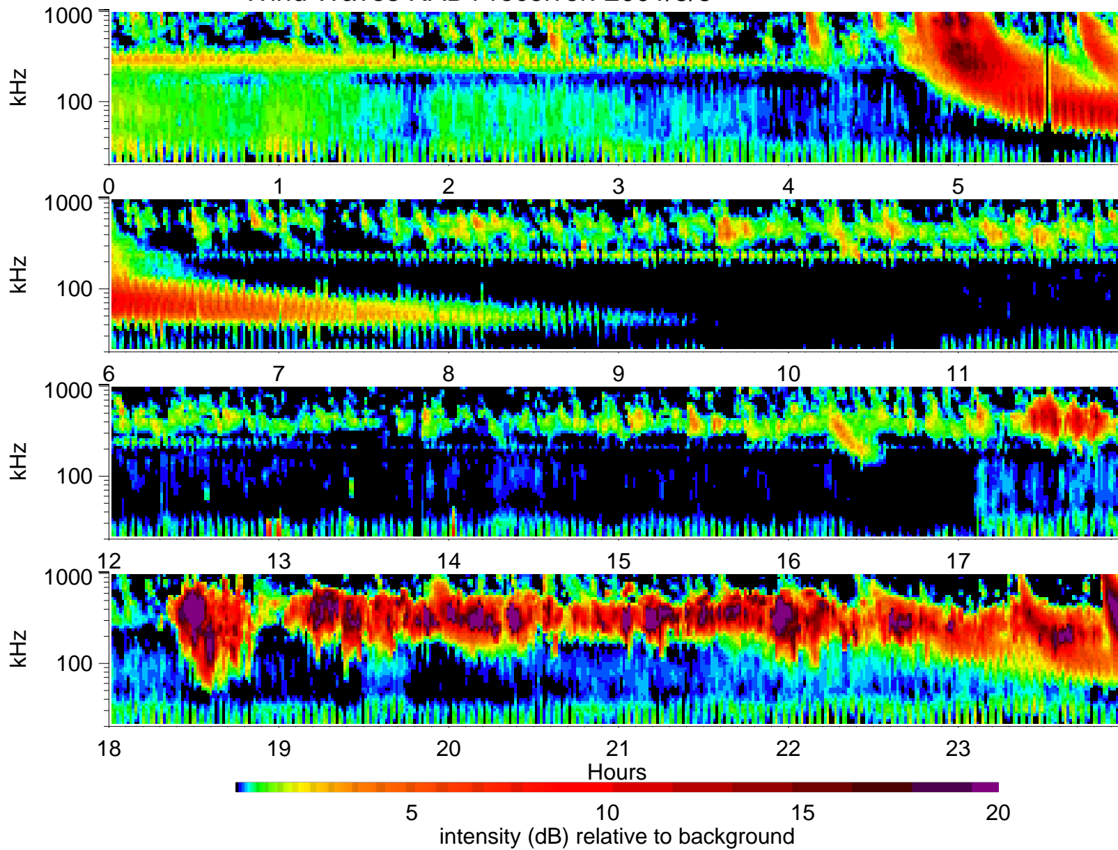
Wind Waves RAD1 receiver: 2001/5/5
