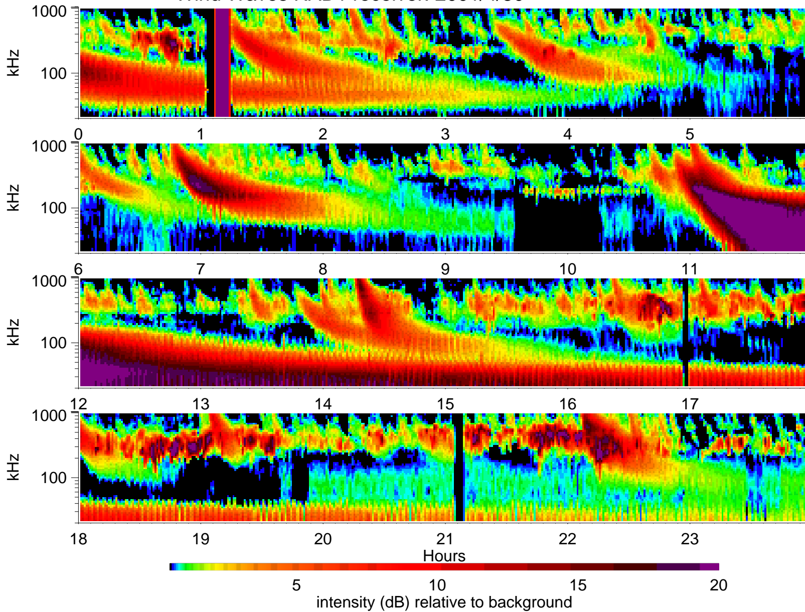
Wind Waves RAD1 receiver: 2001/4/30
