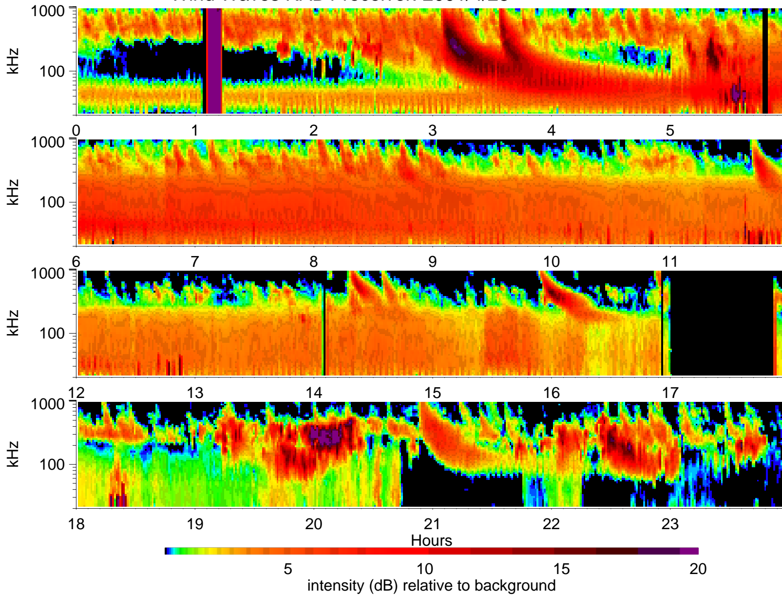
Wind Waves RAD1 receiver: 2001/4/28
