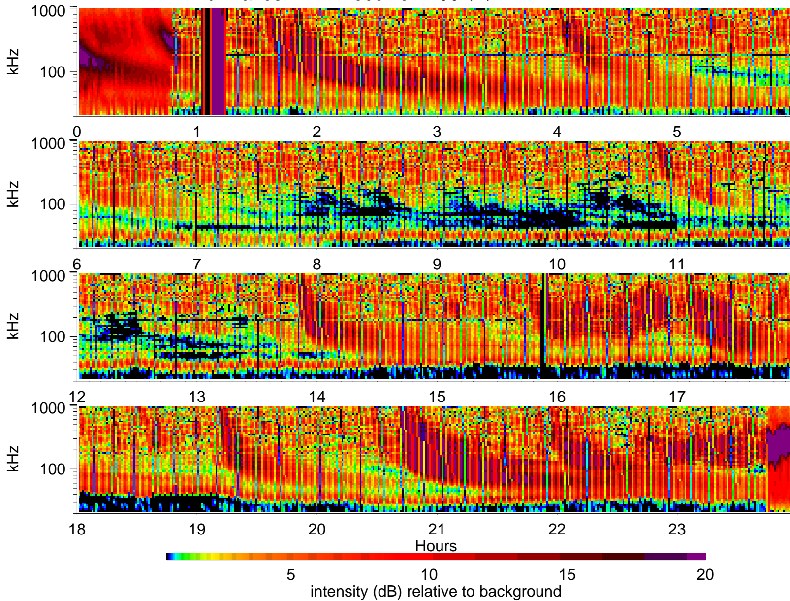
Wind Waves RAD1 receiver: 2001/4/22
