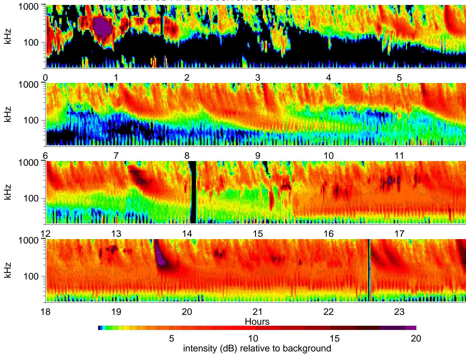
Wind Waves RAD1 receiver: 2001/4/21
