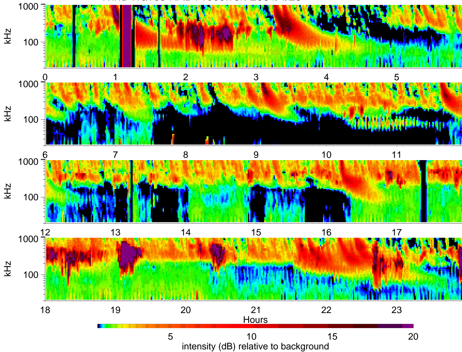
Wind Waves RAD1 receiver: 2001/4/20
