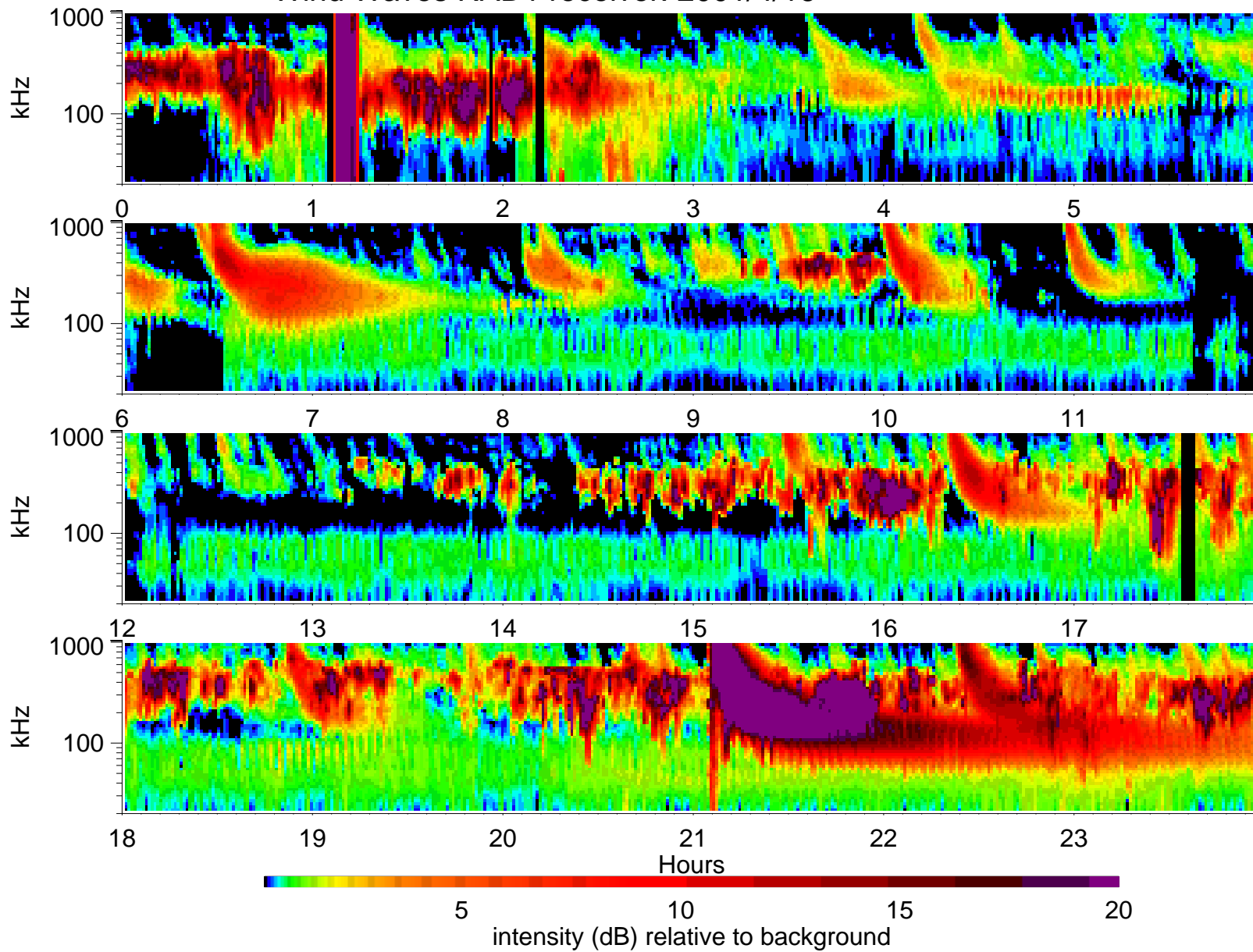
Wind Waves RAD1 receiver: 2001/4/16
