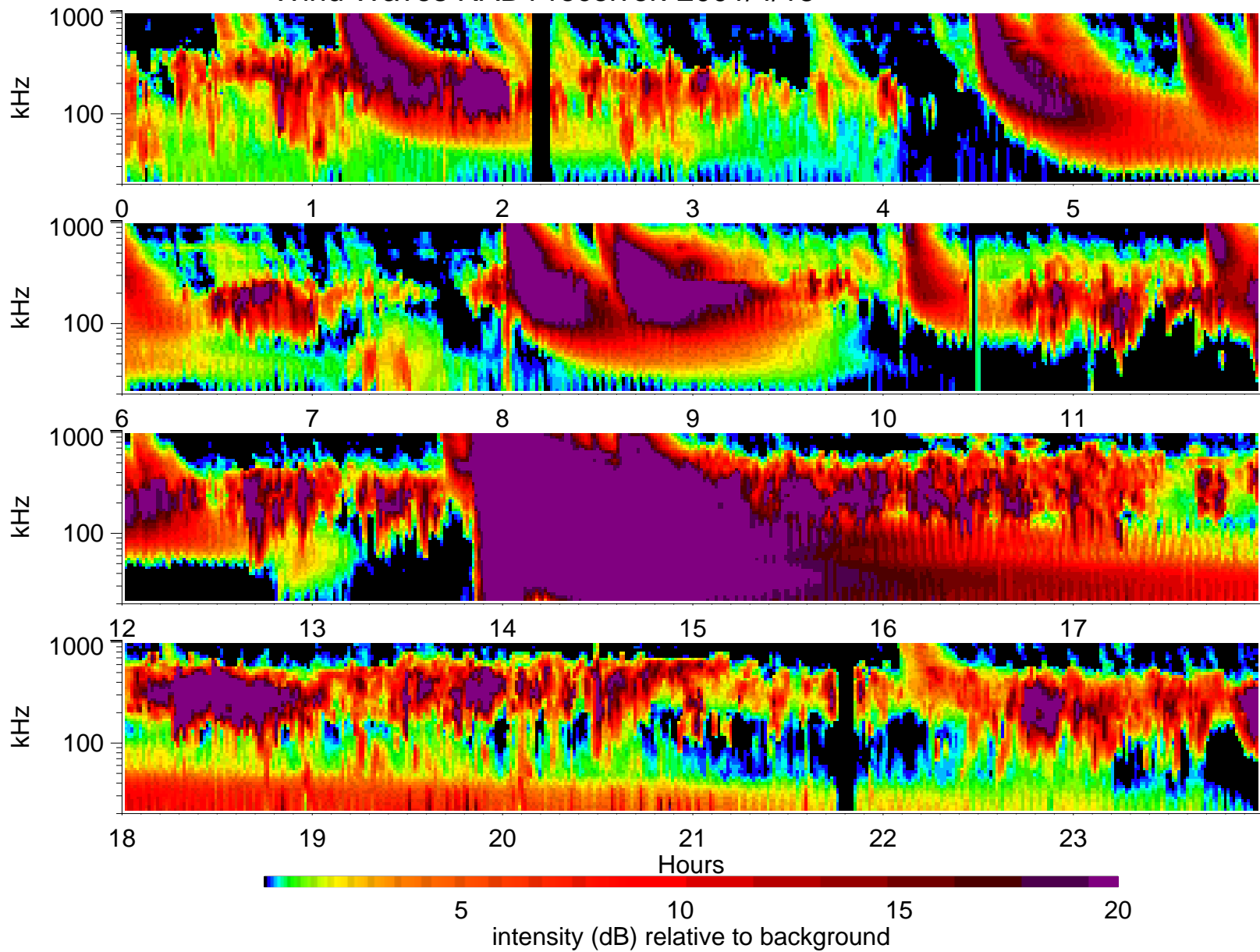
Wind Waves RAD1 receiver: 2001/4/15
