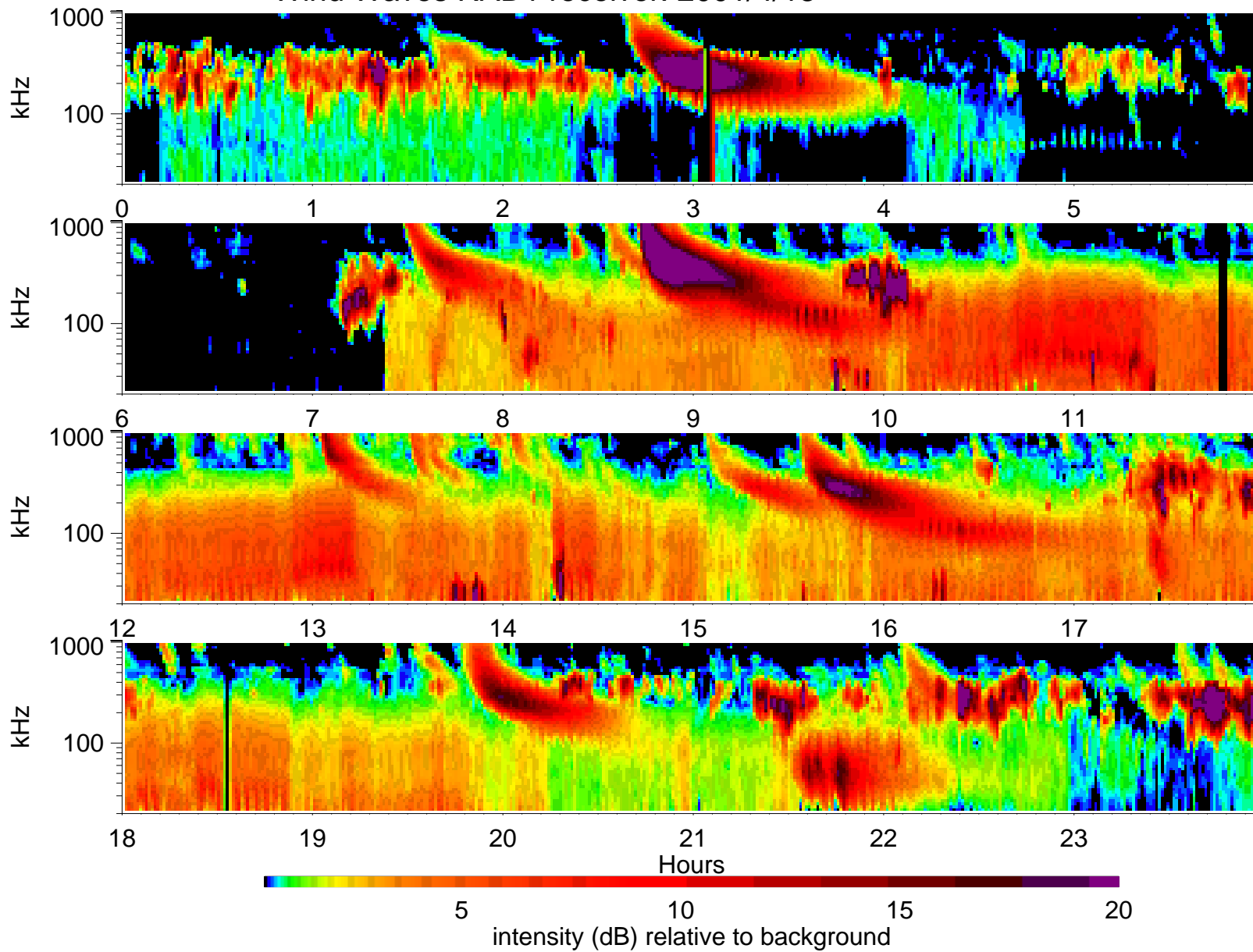
Wind Waves RAD1 receiver: 2001/4/13
