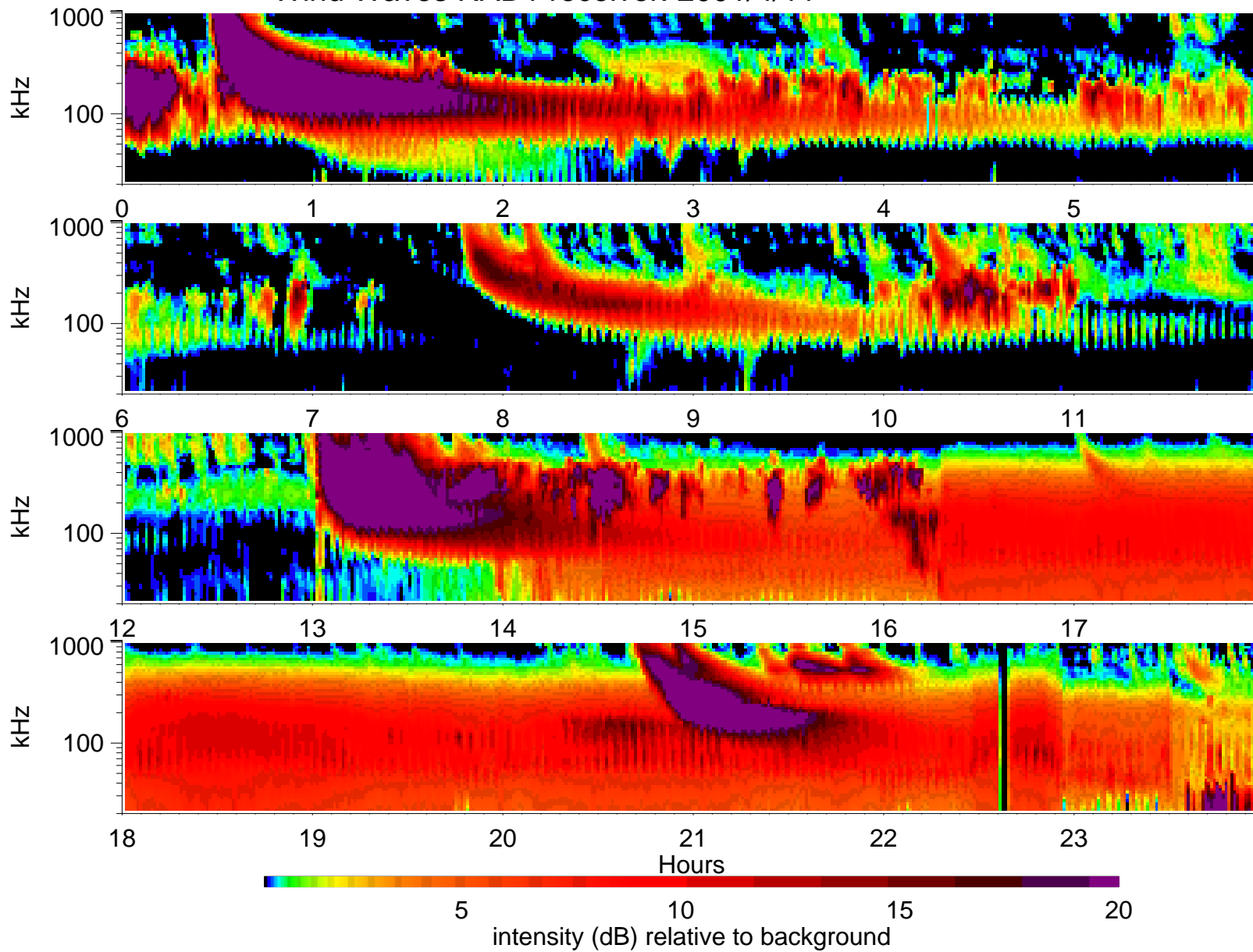
Wind Waves RAD1 receiver: 2001/4/11
