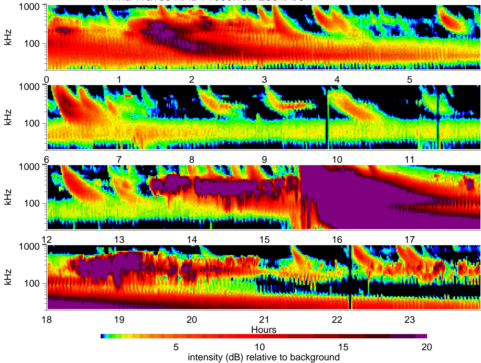
Wind Waves RAD1 receiver: 2001/4/9
