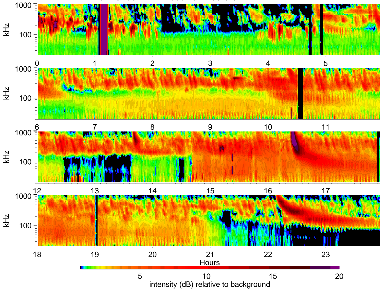
Wind Waves RAD1 receiver: 2001/4/4
