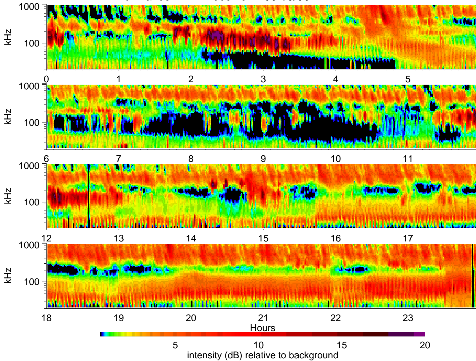
Wind Waves RAD1 receiver: 2001/3/30
