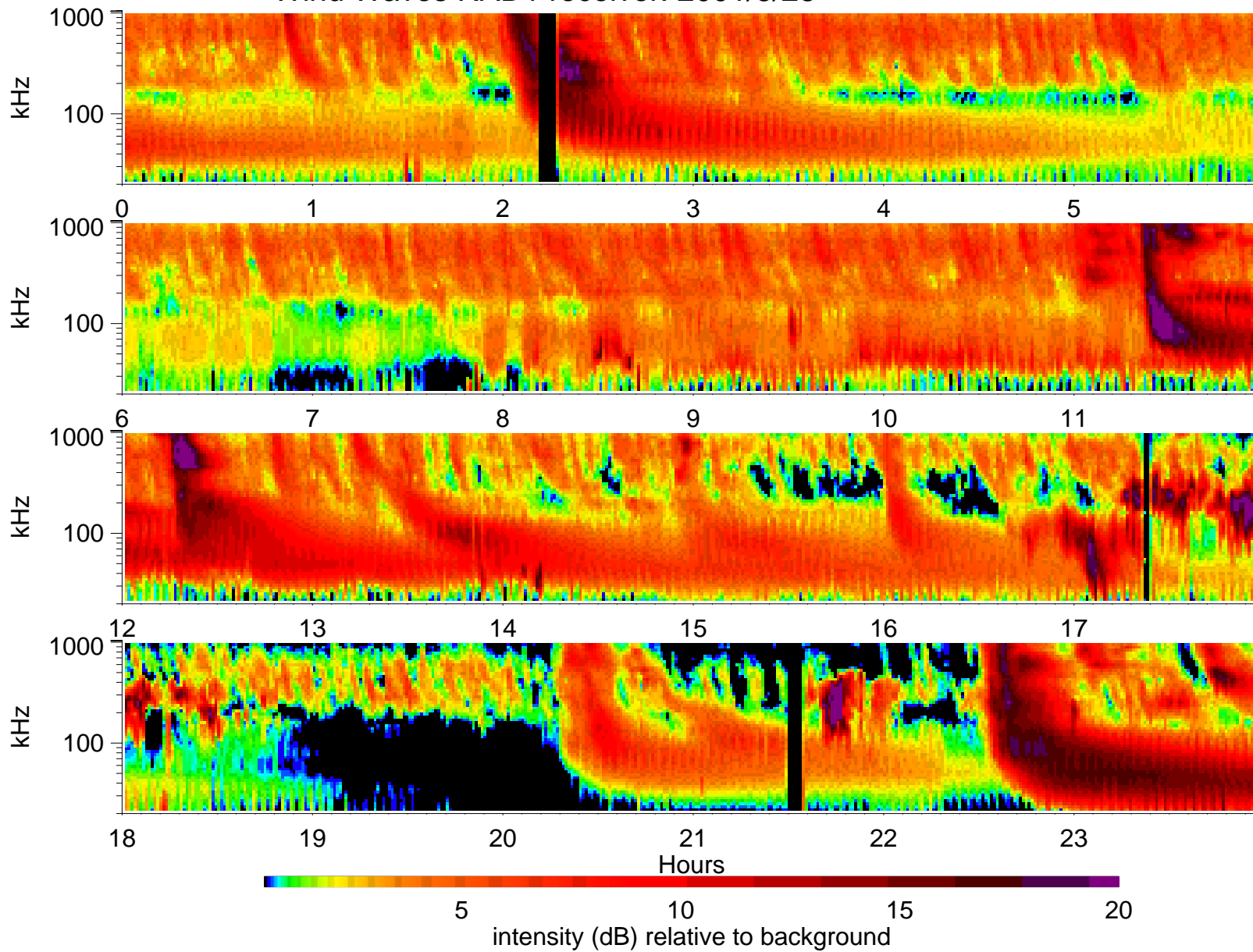
Wind Waves RAD1 receiver: 2001/3/28
