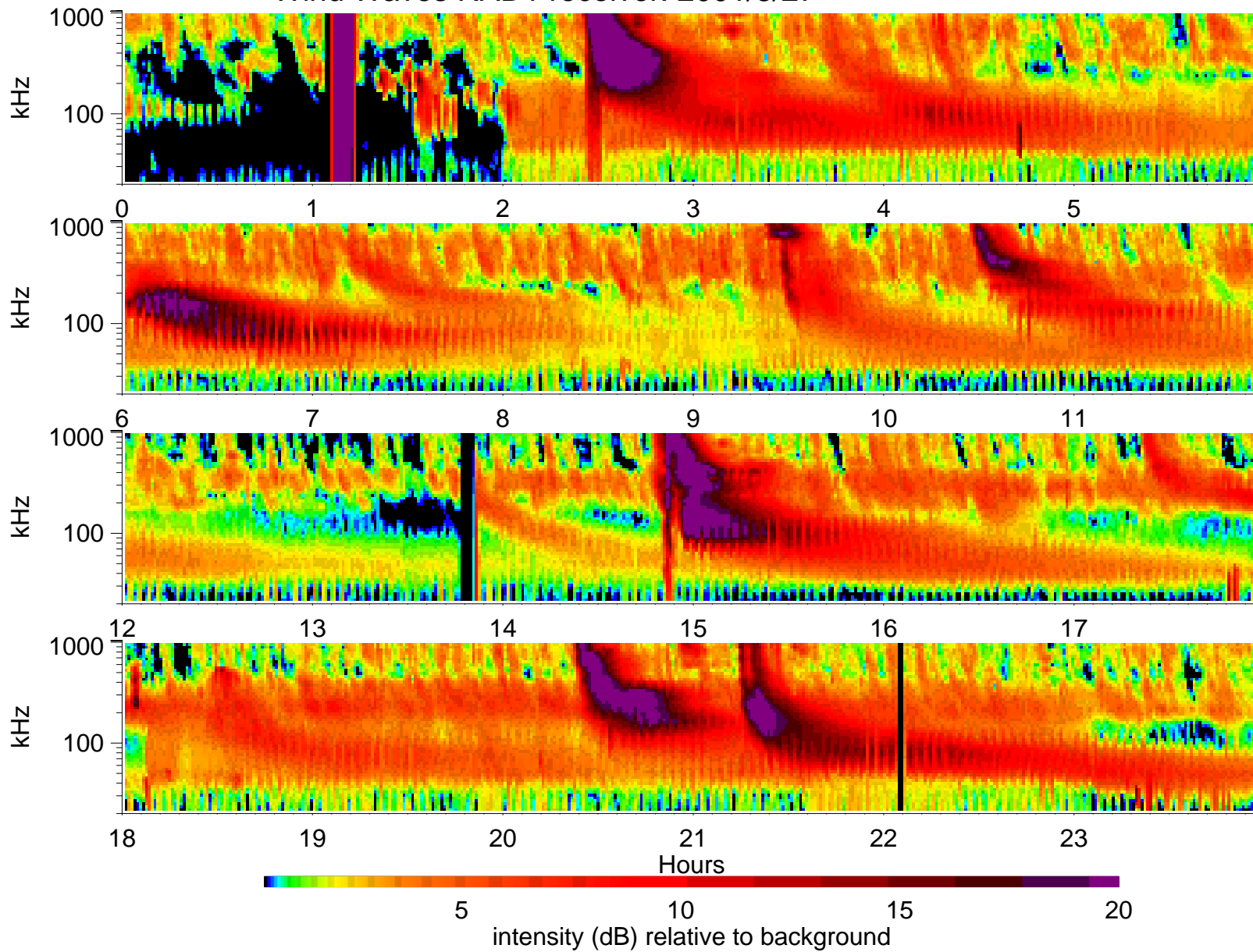
Wind Waves RAD1 receiver: 2001/3/27
