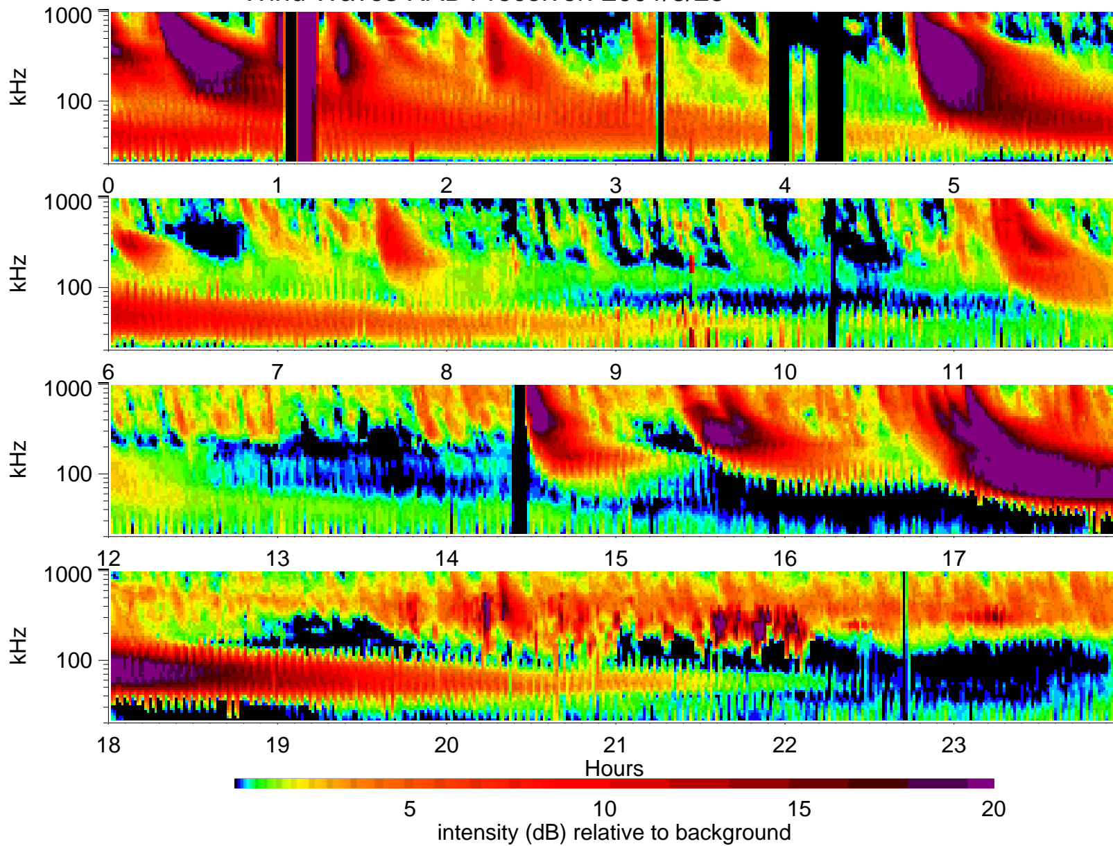
Wind Waves RAD1 receiver: 2001/3/25
