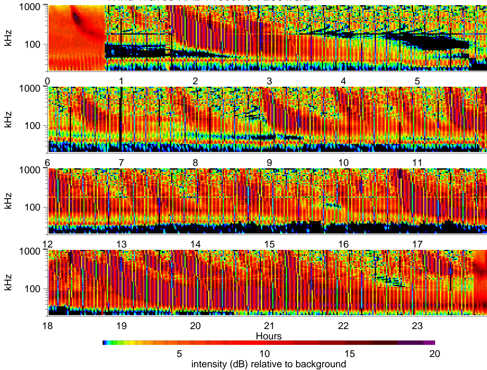
Wind Waves RAD1 receiver: 2001/3/24
