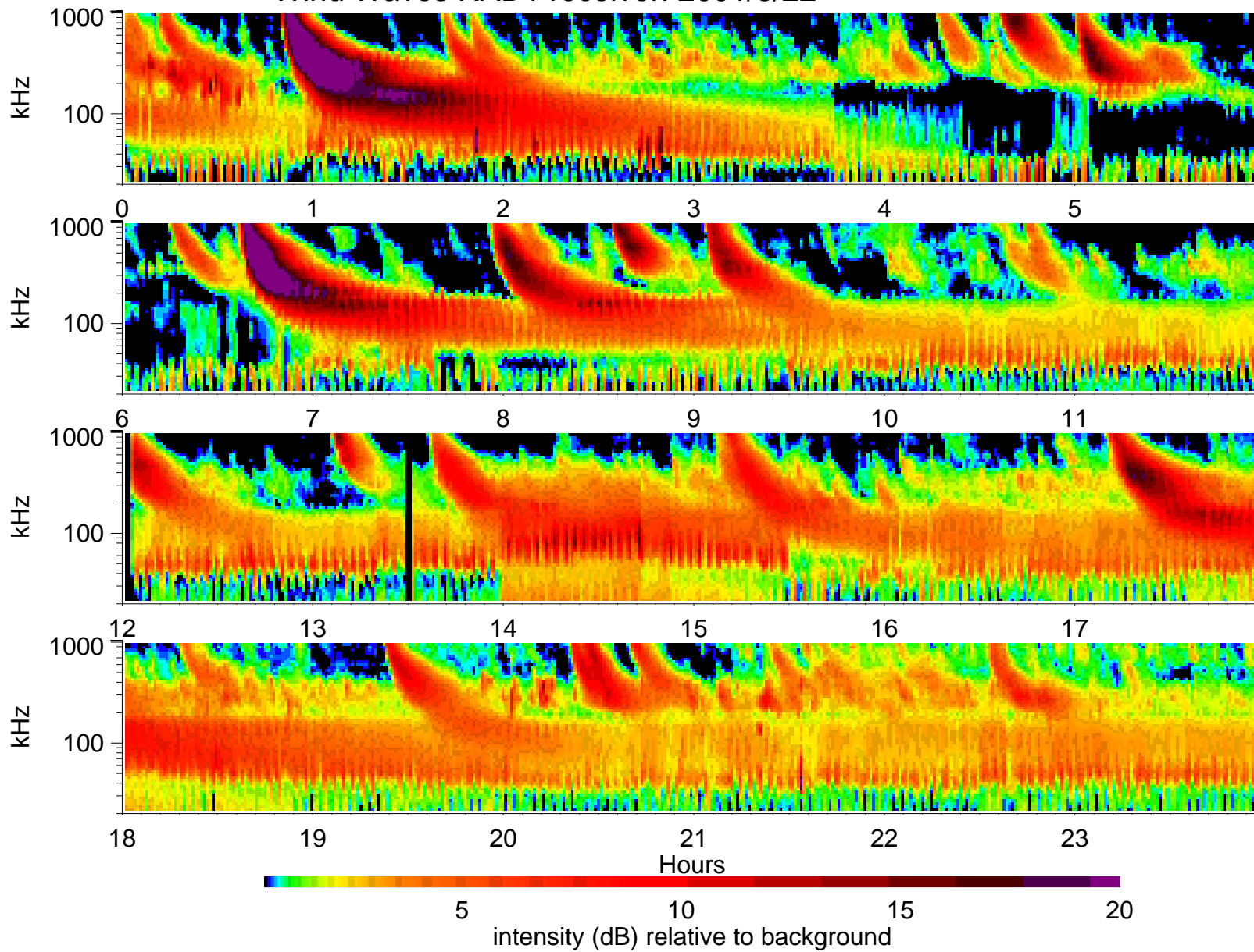
Wind Waves RAD1 receiver: 2001/3/22
