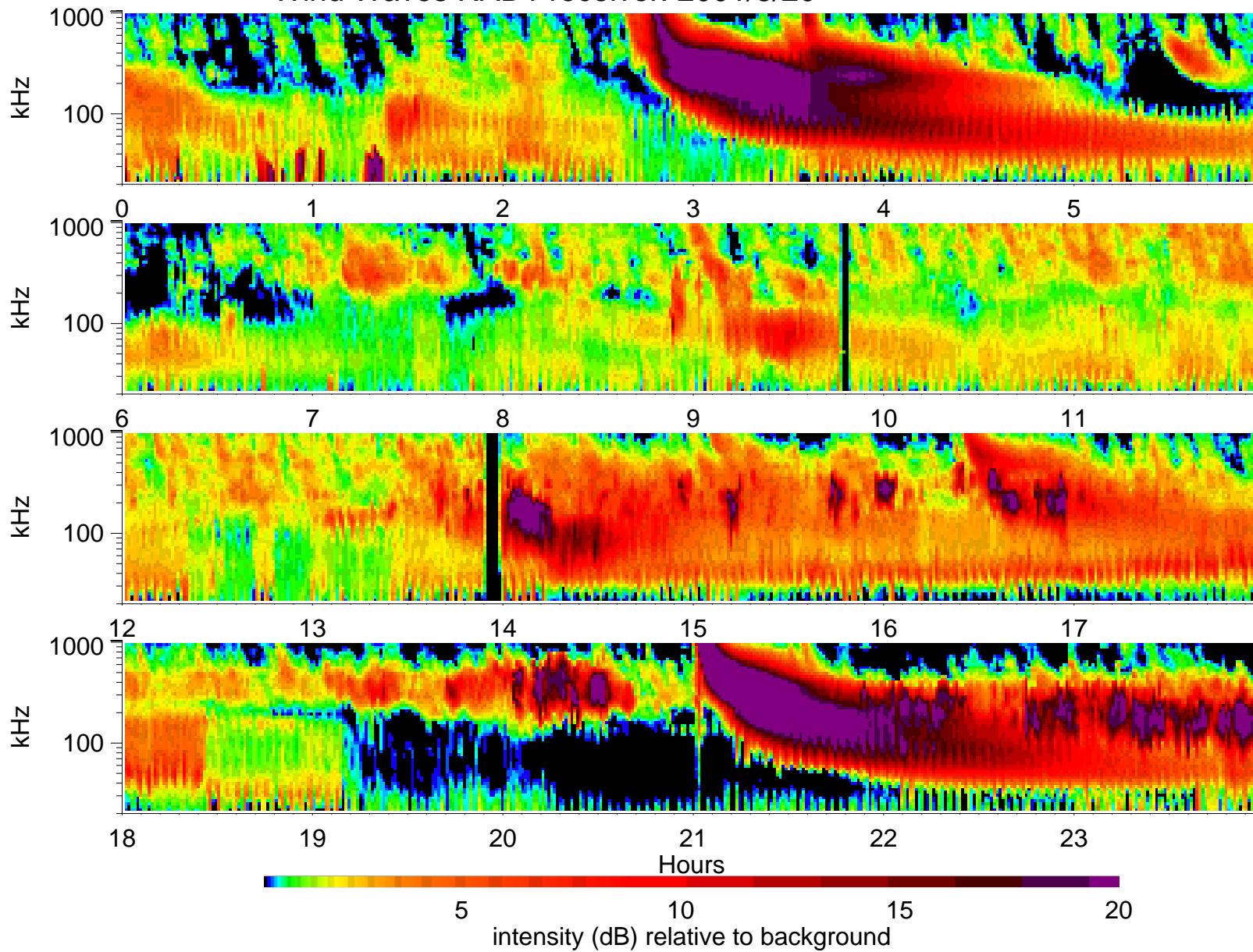
Wind Waves RAD1 receiver: 2001/3/20
